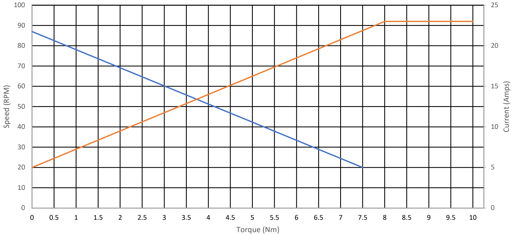
Motor Performance Curve @ 14.0 Volts And 25° C
